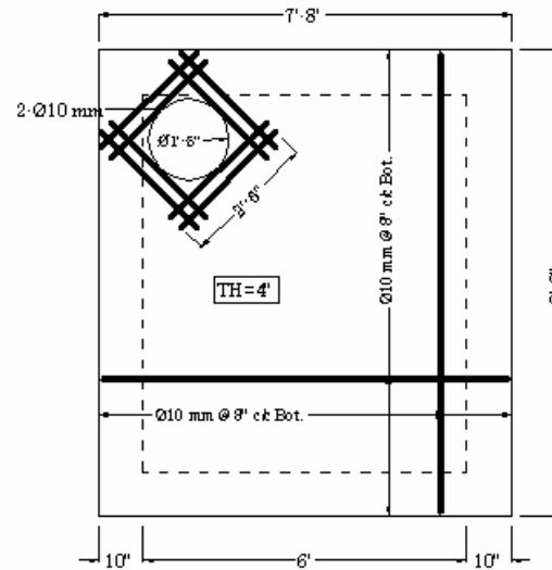
RESERVOIR TOP SLAB
