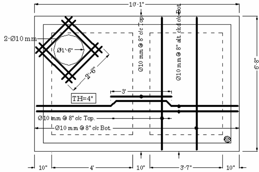
RESERVOIR TOP SLAB
