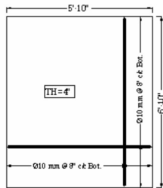
BATHING/ WASHING PLATFORM (IF REQUIRED)
