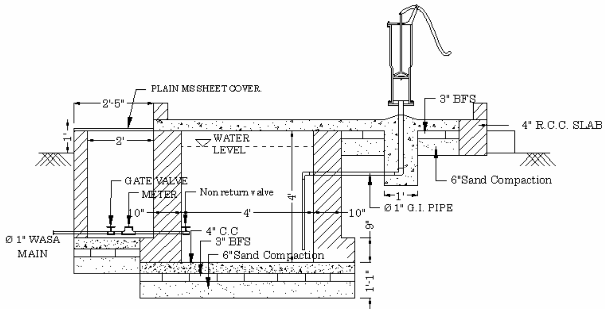
SECTION AA
